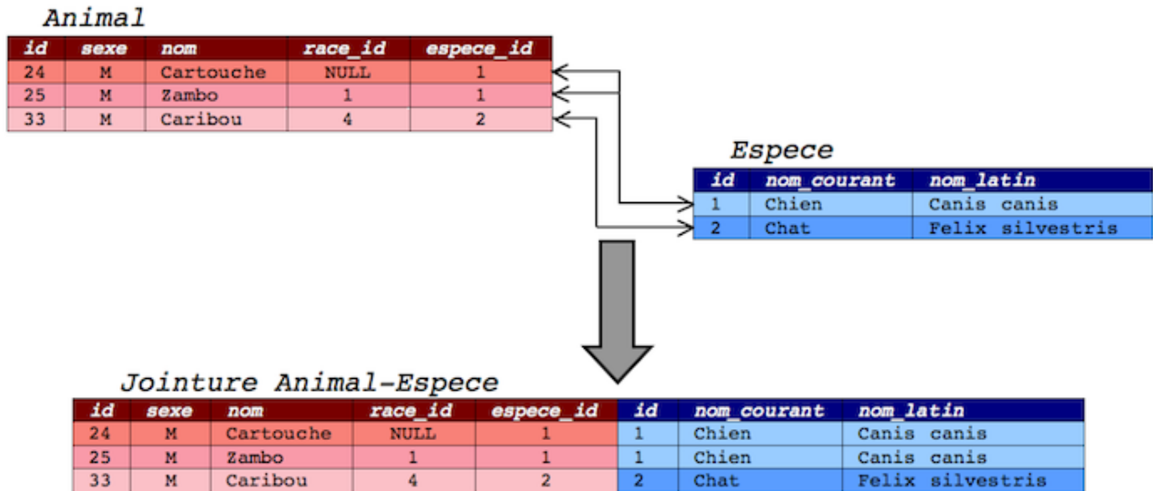
FIGURE II.3.1. – Principe des jointures
